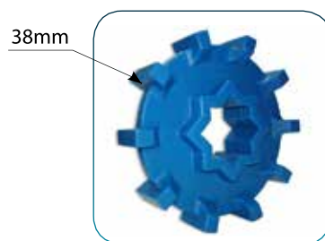
Molded Sprockets made of Acetal
