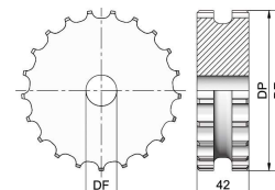
Solid Idler Wheel
